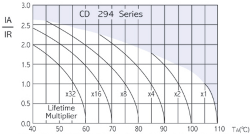
寿命曲线 Lifetime Diagram
